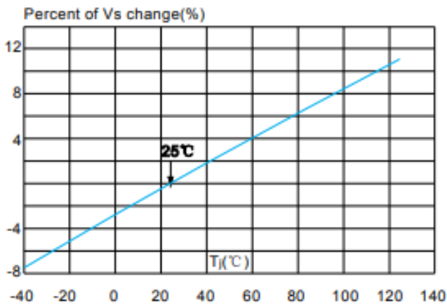
FIGURE 1 Normalized VS. Change VS. Junction Temperature
