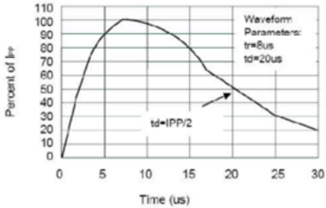
FIGURE 1 Pulse Waveform
