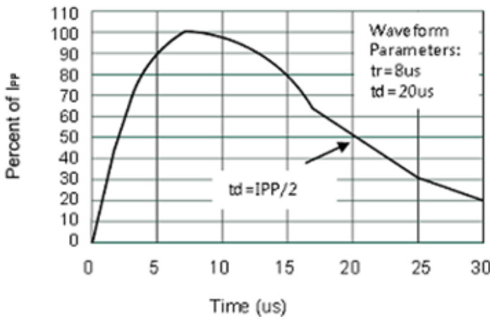
FIGURE 1 Pulse Waveform
