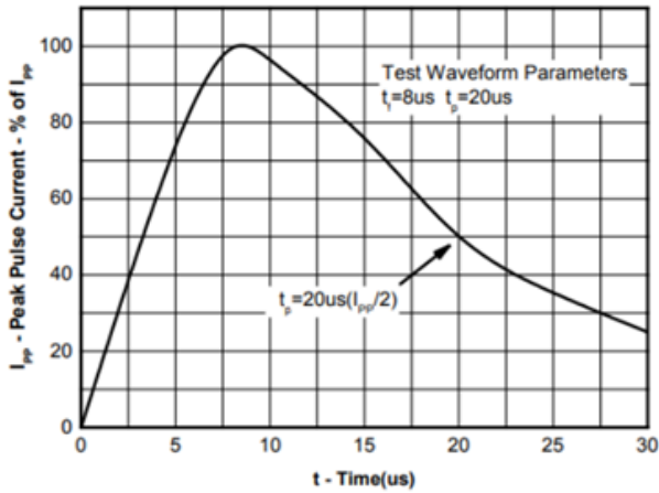
FIGURE 1 Pulse Waveform
