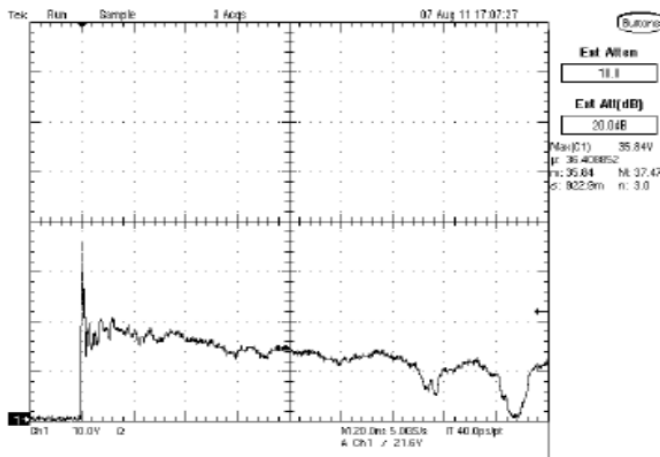
FIGURE 3 ESD clamping voltage screenshot Positive 8 kV contact per IEC61000-4-2
