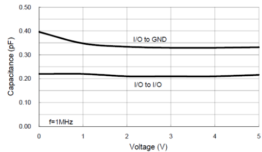
FIGURE 4 Voltage VS. Capacitance
