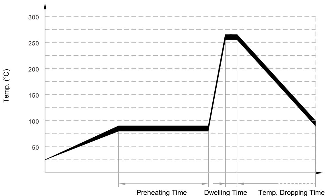
Wave Soldering Curve
